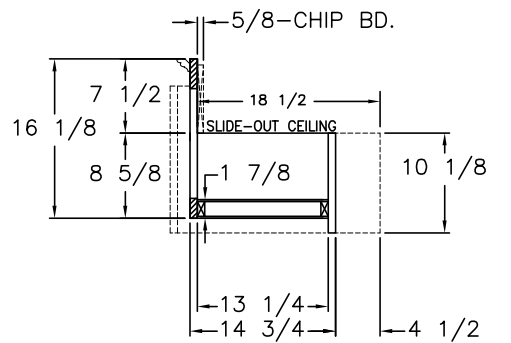
SIDE SECTION B
