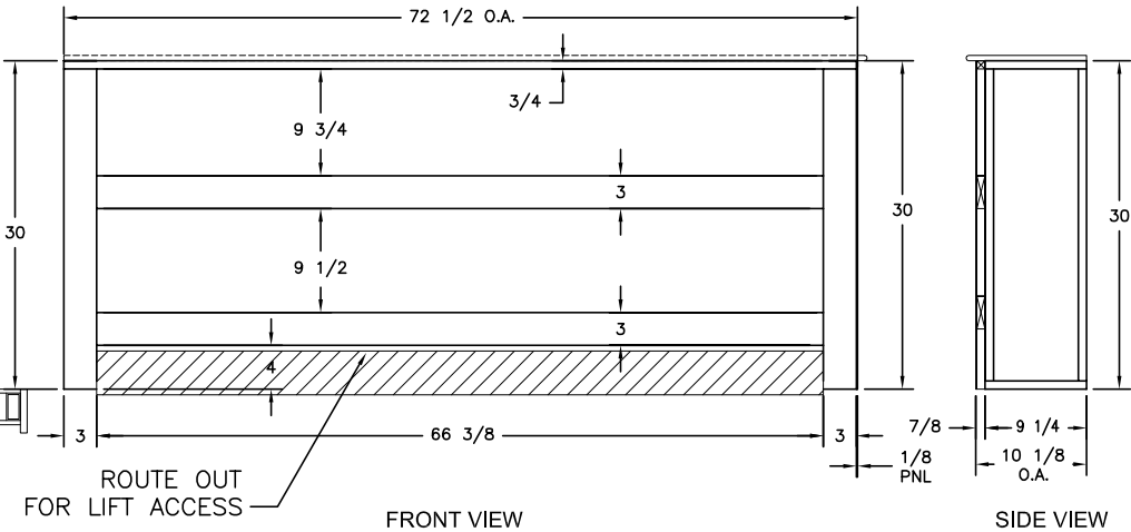
FRONT VIEW
