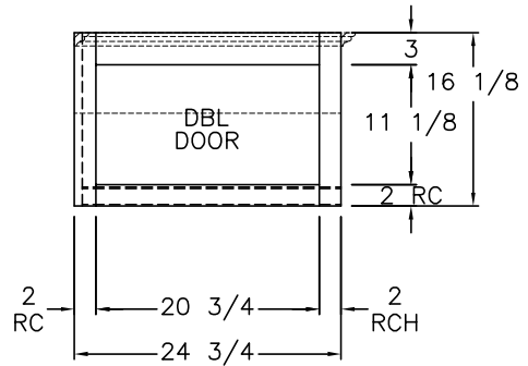
FRONT VIEW A (2) 10 7/8 X 12 1/8 DOORS
