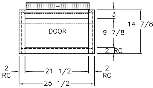
FRONT VIEW B (1) 22 1/2 X 10 7/8 DOOR (PLEXI) (TOP HINGE)
