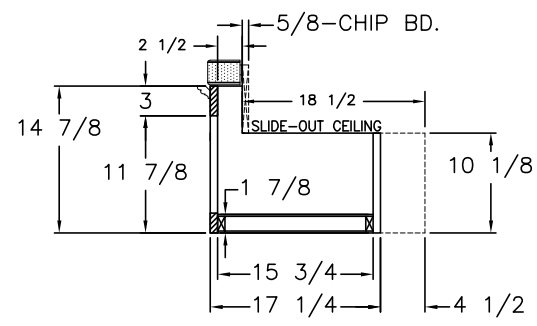
SIDE SECTION A
