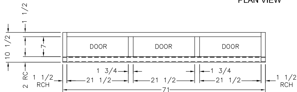
FRONT VIEW (3) 22 x 8 DOORS (TOP HG)
