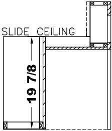
SIDE SECTION (P)
