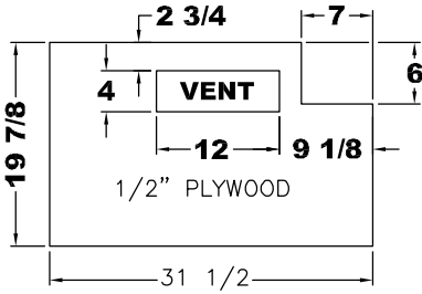
MICROWAVE BACK DETAIL
