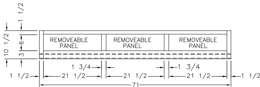
BACK (REAR VIEW)
