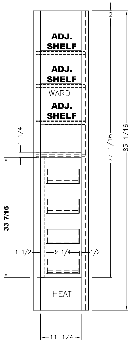
FRONT VIEW (1) 12 1/4x72 5/8 DOOR
