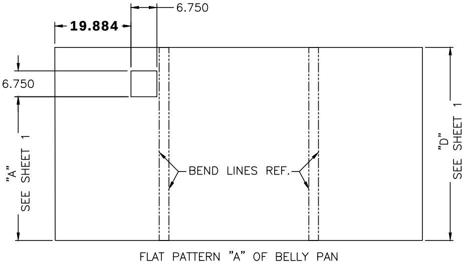
FLAT PATTERN "A" OF BELLY PAN
