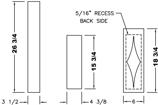
3/4 HARDWOOD 1/4 LAUAN FABRIC WRAPPED 3/4 HARDWOOD
