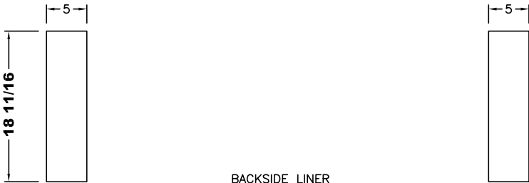
BACKSIDE LINER MAT'L: .080 ABS - P/N 108200
