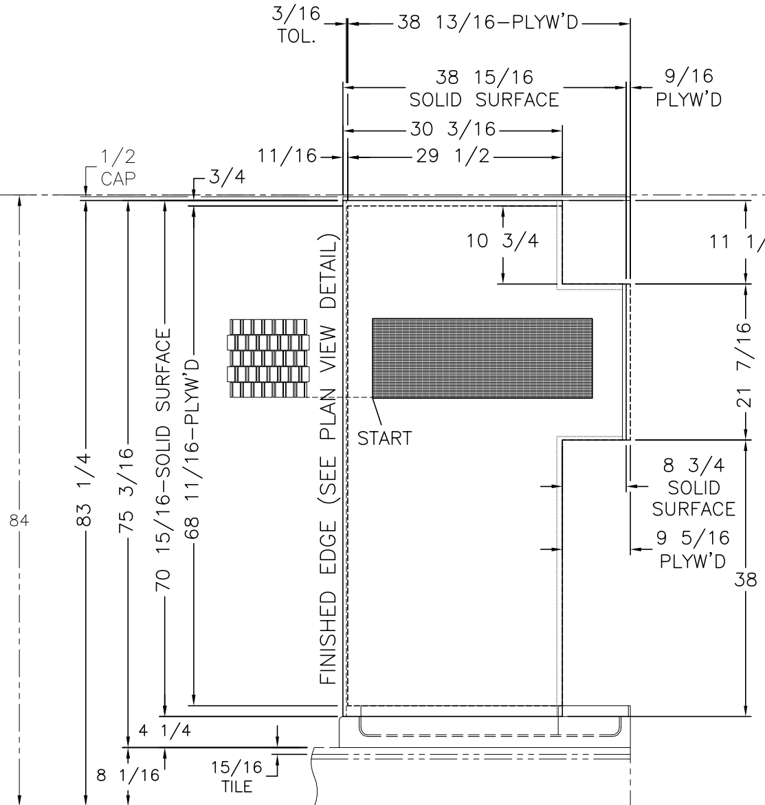
VIEW (A)
