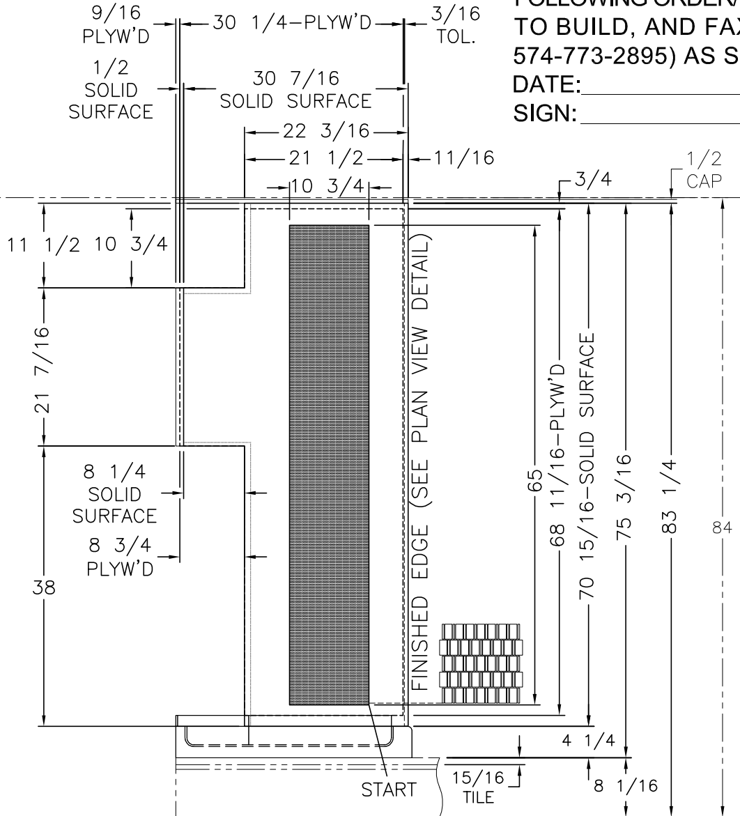
VIEW (B)
