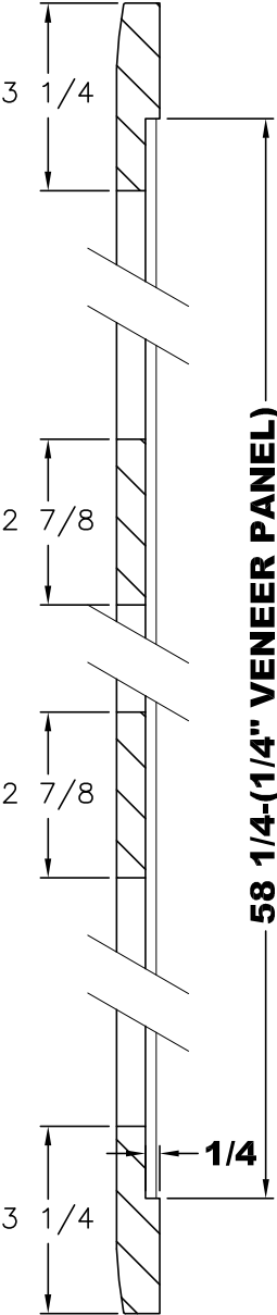
C-C (ENLARGED 5X)
