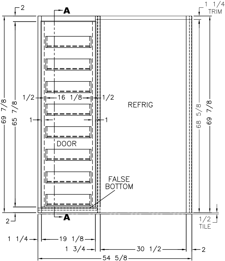
FRONT VIEW (1) 17 3/8x66 5/8 DOOR
