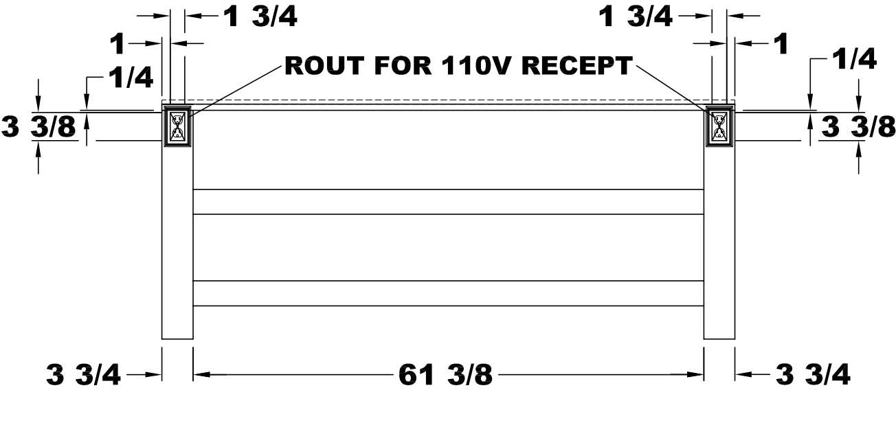
FRONT VIEW (FRAME)
