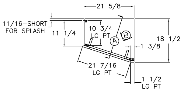
TOP VIEW 16 7/16Wx14 3/4H TAMBOUR DOOR
