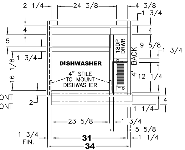
VIEW B
