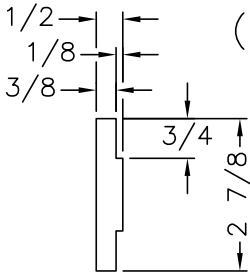
TYPICAL INTERIOR/ HORIZONTAL RAILS
