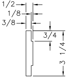
INTERIOR VERTICAL RAIL
