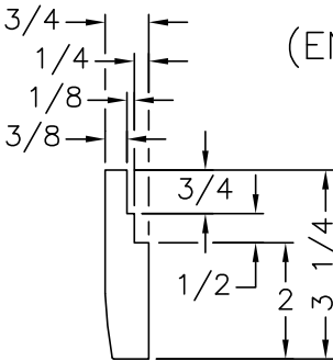
TYPICAL PERIMETER RAILS
