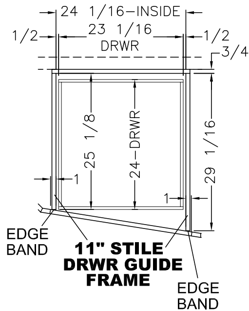
PULLOUT DRAWER DETAIL
