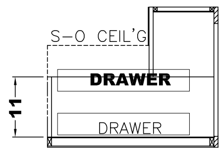
SIDE SECTION (B)
