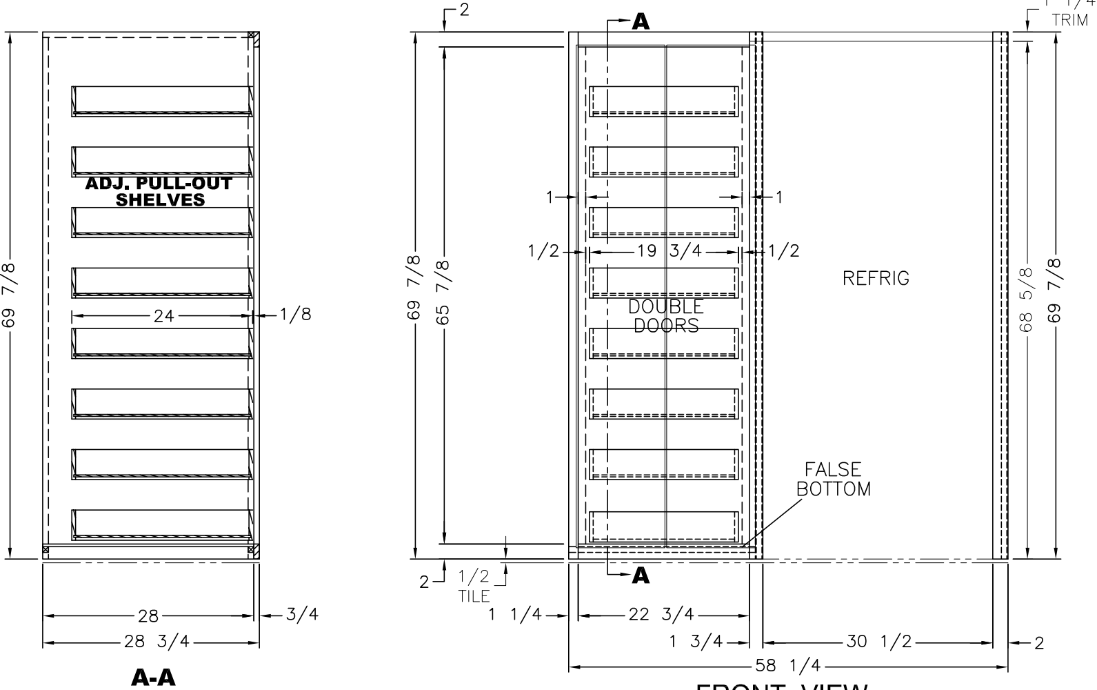
FRONT VIEW (2) 11 3/4x66 5/8 DOORS
