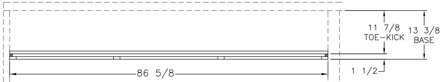
TOP VIEW
