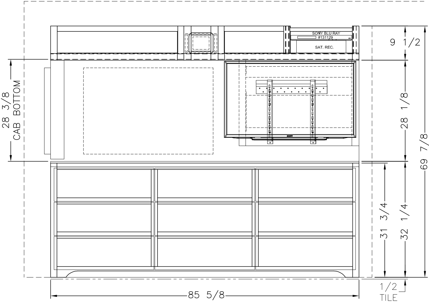
FRONT VIEW
