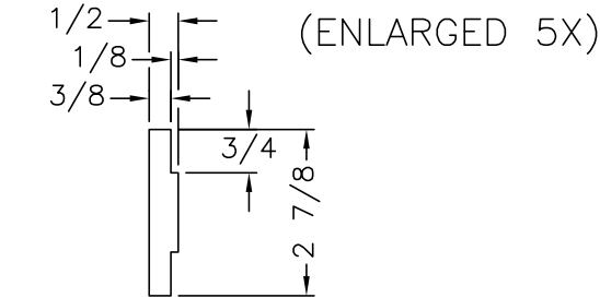
TYPICAL INTERIOR/ HORIZONTAL RAILS
