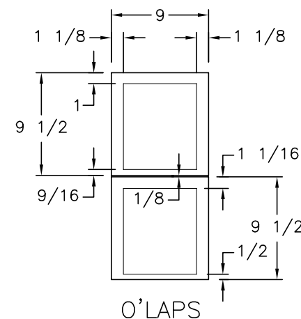
(2) 9 1/2x9 FRONTS
