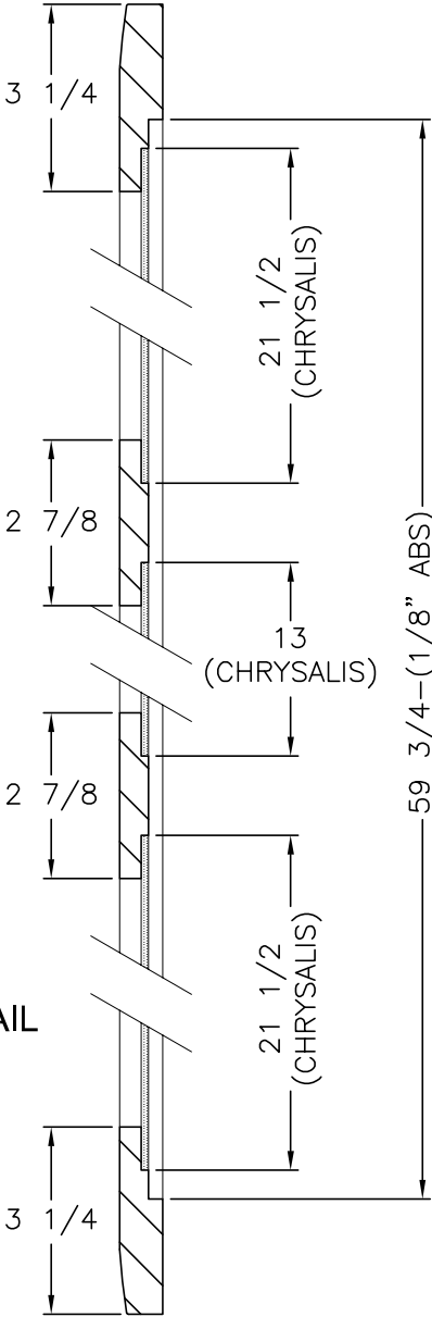
C-C (ENLARGED 5X)
