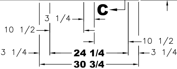
SLIDING DOOR (2) REQ'D
