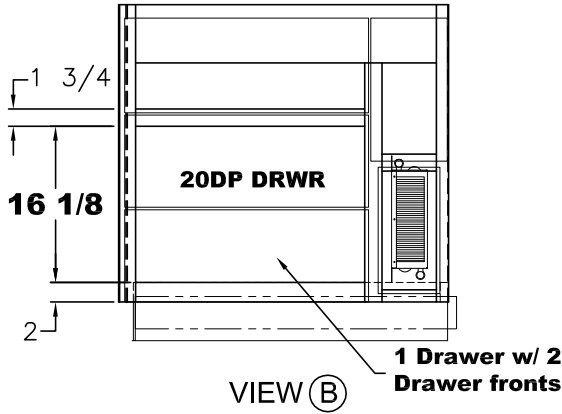
(2) 9 1/2x25 1/8 DRAWER FRONTS
