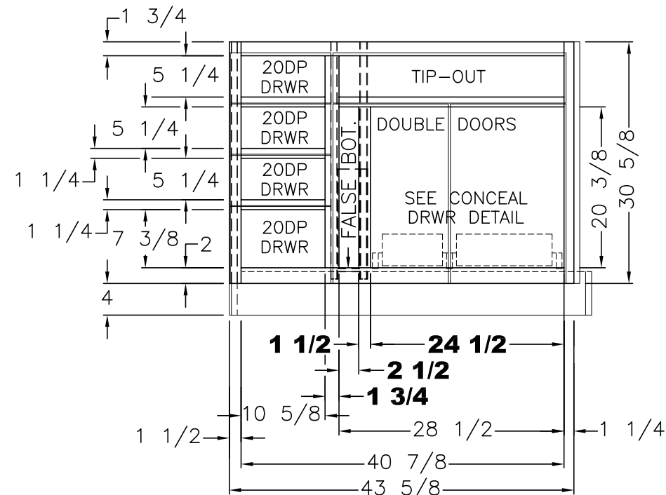
VIEW (A)
