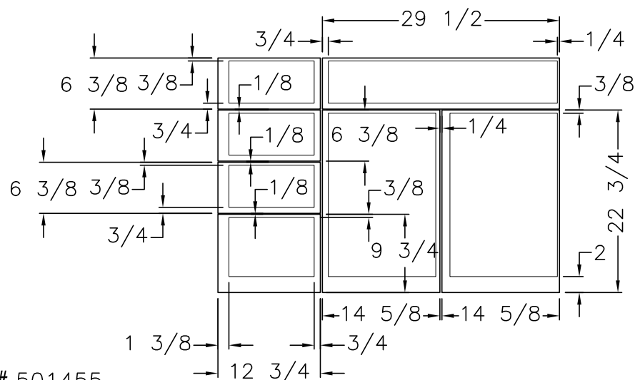
VIEW A OVERLAPS
