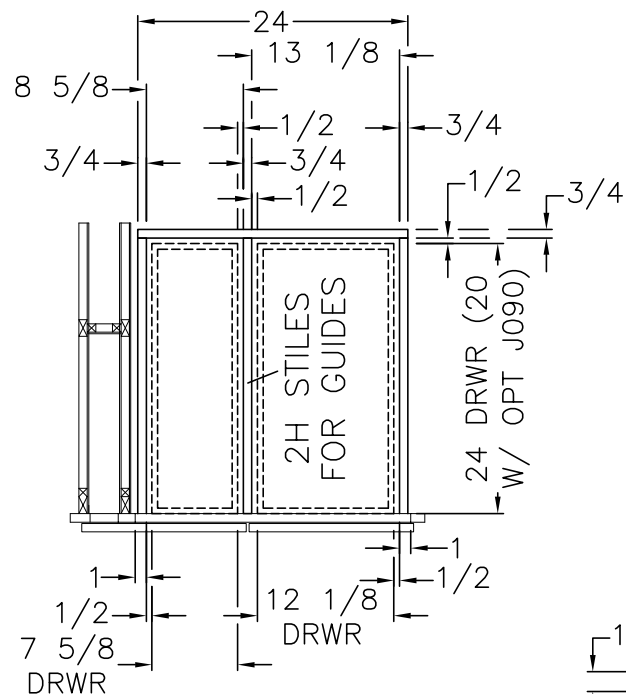
VIEW A DRAWER DETAIL
