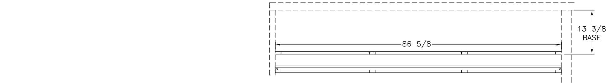
TOP VIEW TOP TIER
