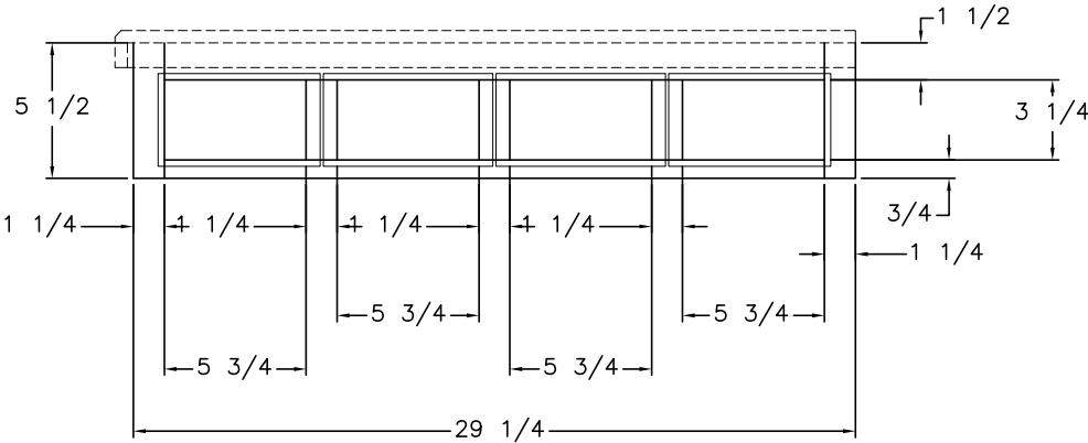
FRONT VIEW (2X SCALE)
