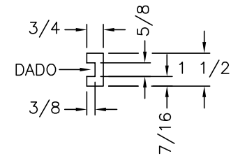
HARDWOOD TRACK DETAIL (2X SCALE)
