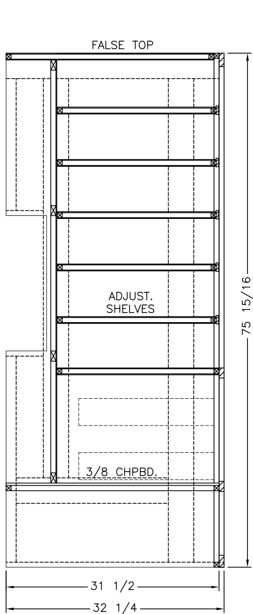
SECTION VIEW (A)
