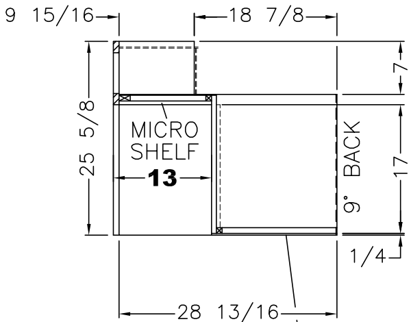
BOTTOM PANEL BACK OF MICROWAVE VIEW (L)
