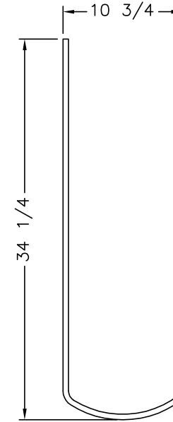
COUNTERTOP AND EDGE TREATMENT
