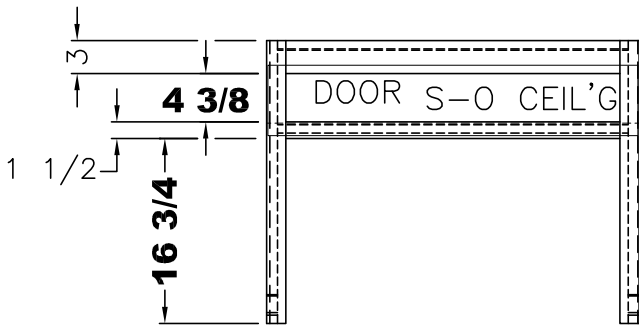
VIEW (F) (1) 33 1/2x6 3/8 DOOR (TOP HG)
