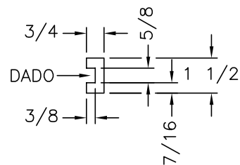
HARDWOOD TRACK DETAIL (2X SCALE)
