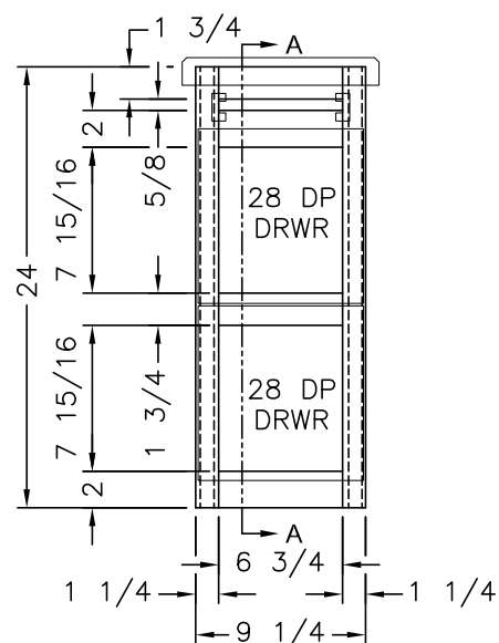
(2) 9 1/2 X 9 FRONTS FRONT VIEW
