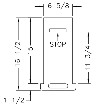
1/2" SOLID SURFACE P-O SHELF
