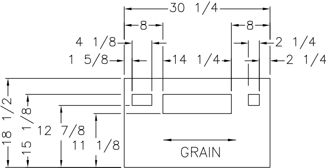
5/8 PLYWOOD DETAIL
