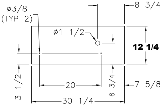
1/2" PLYWOOD MICRO SHELF
