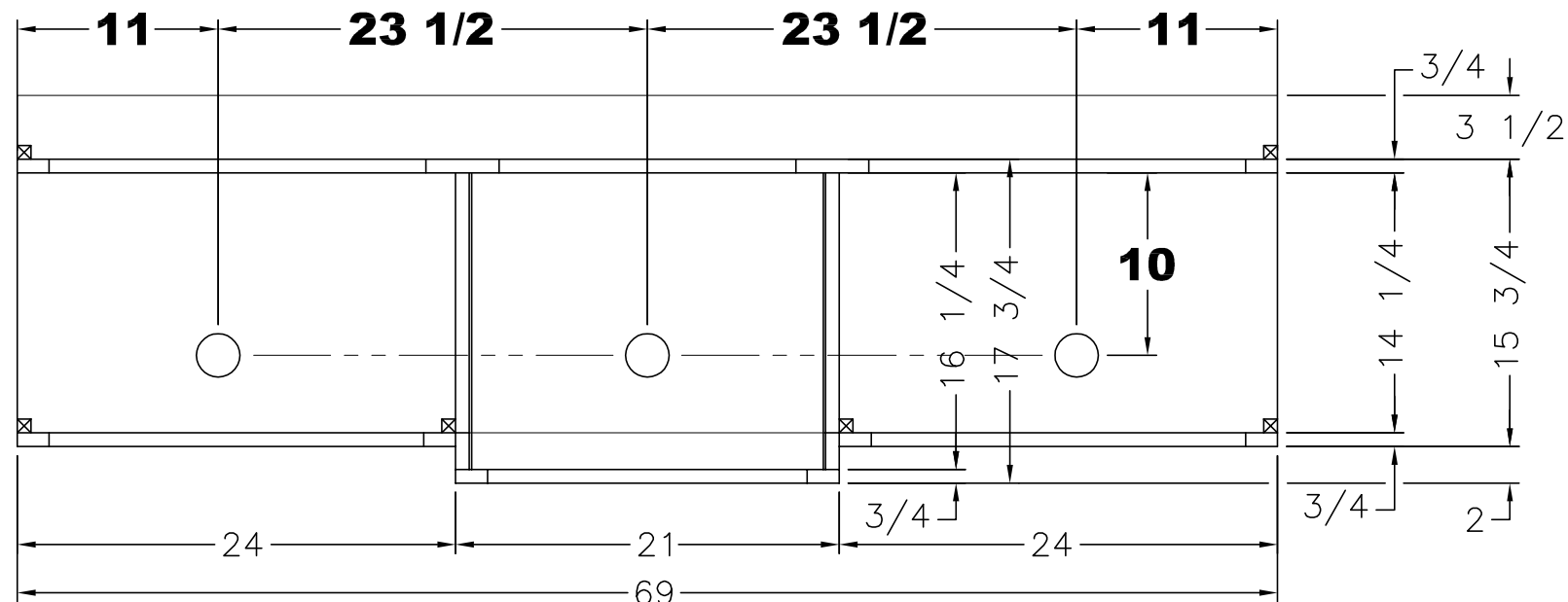
PLAN VIEW
