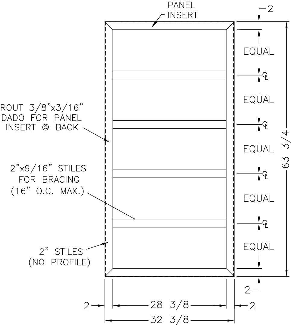
FRAMELESS MIRROR DOOR (2) REQ'D
