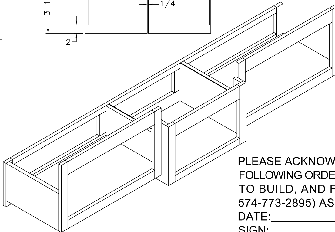
OVERLAPS
