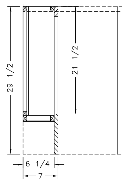
SIDE SECTION (A)
