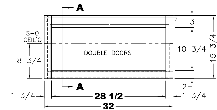
FRONT VIEW (2) 14 5/8x13 1/2 DOORS
