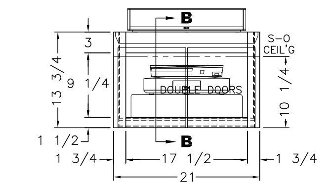
FRONT VIEW (2) 9 3/4x11 1/2 DOORS
