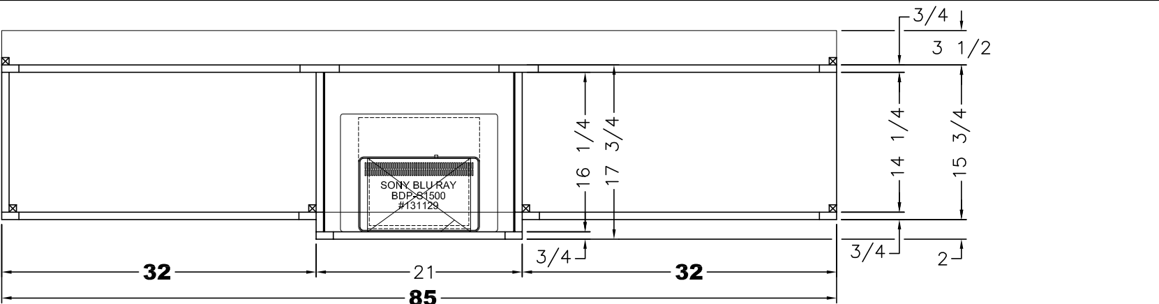
PLAN VIEW
