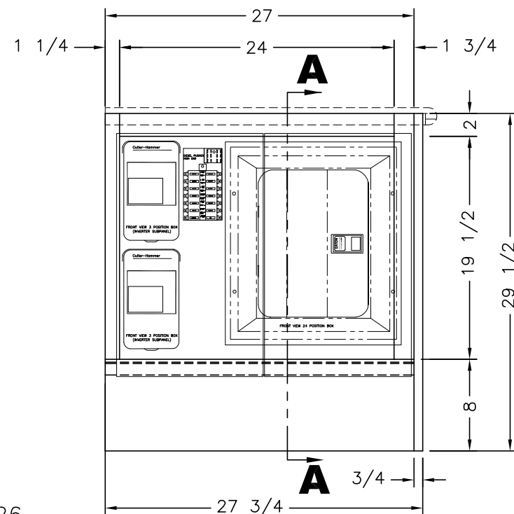
(2) 12 5/8 x 21 1/4 DOORS
