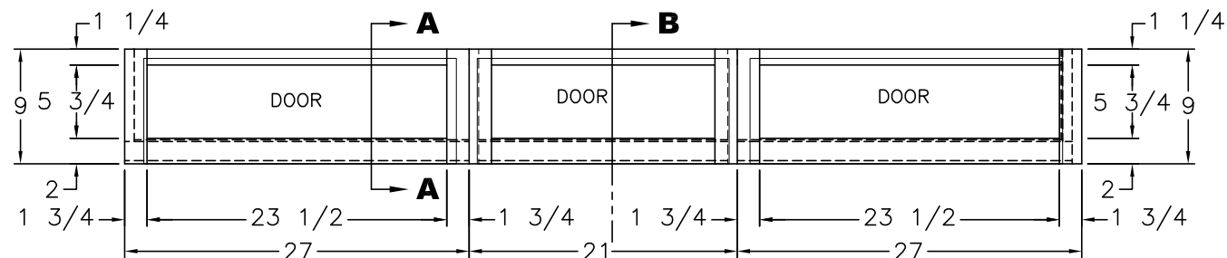
FRONT VIEW
