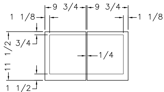
OVERLAPS
