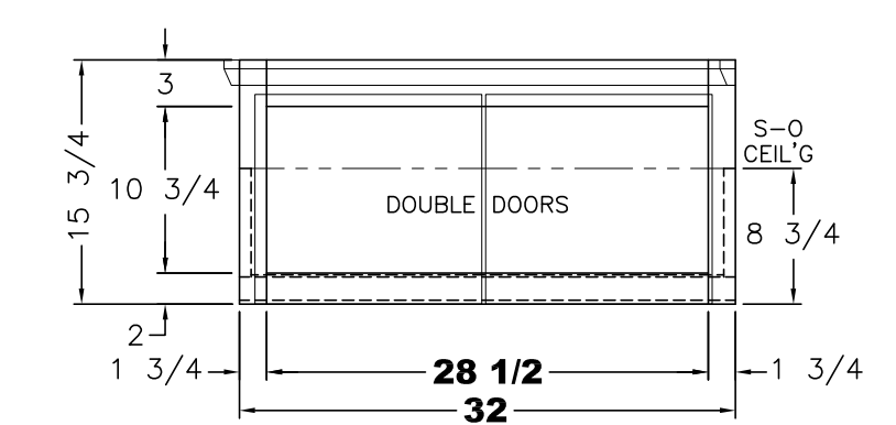
FRONT VIEW (2) 14 5/8x13 1/2 DOORS
