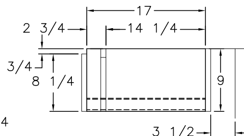
RETURN (2-REQ'D)
