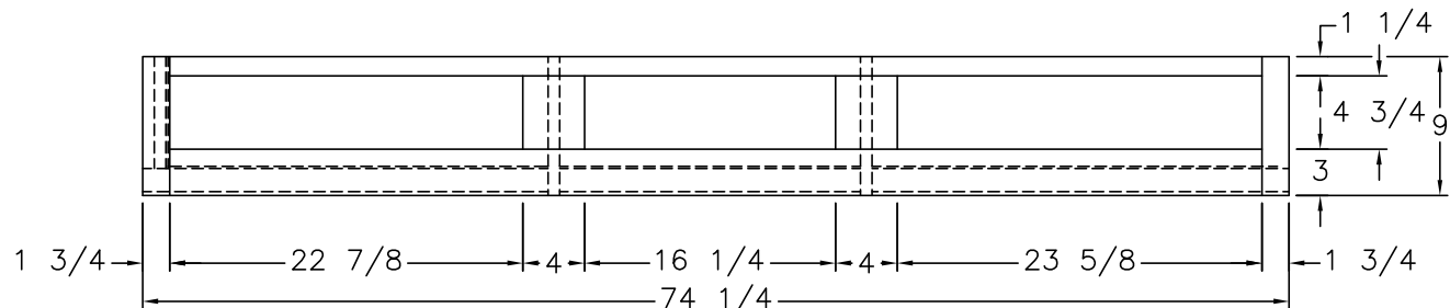
BACK (REAR VIEW)
