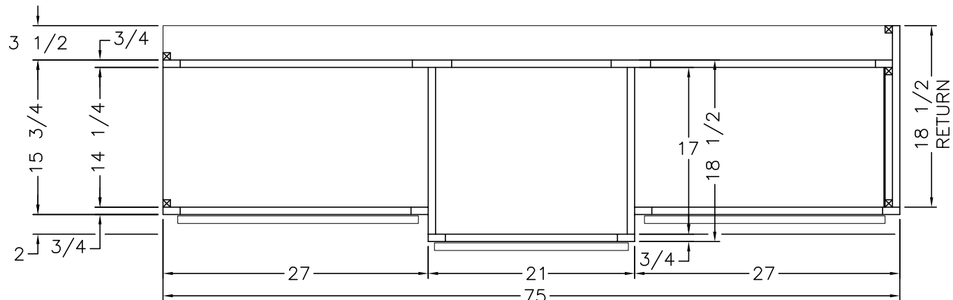
PLAN VIEW
