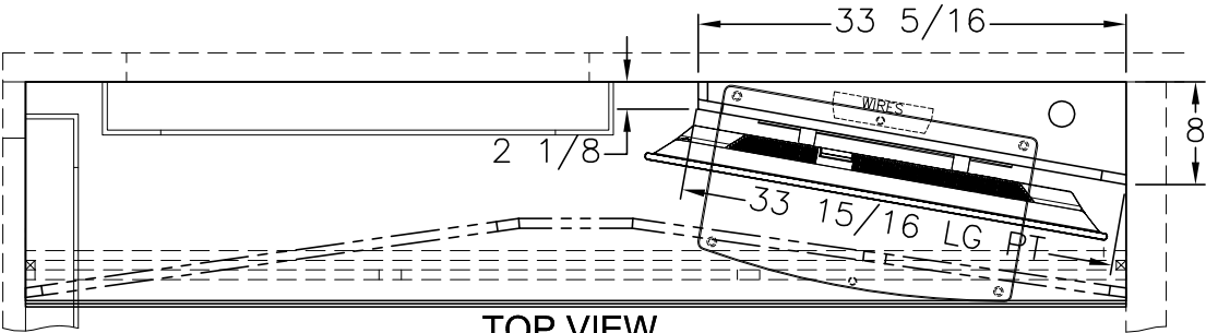
TOP VIEW
