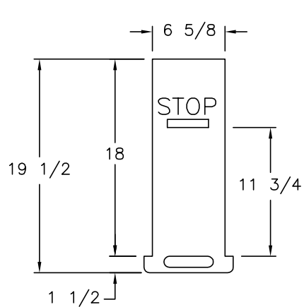
1/2 SOLID SURFACE P-O SHELF
