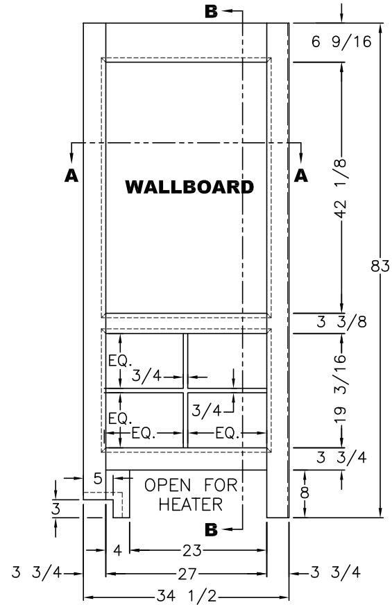
VIEW 'D' PANEL OVERLAY
