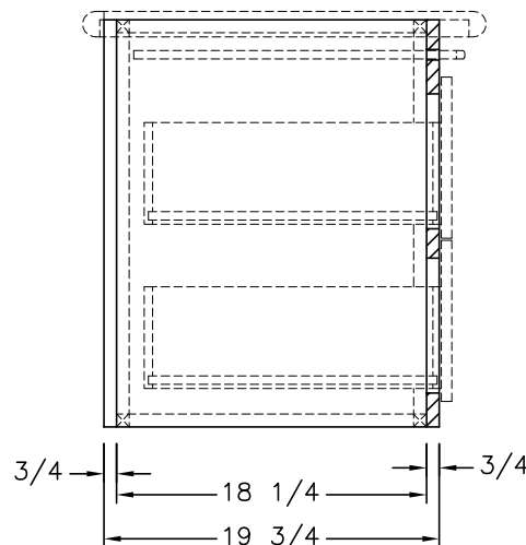
SIDE SECTION (A)
