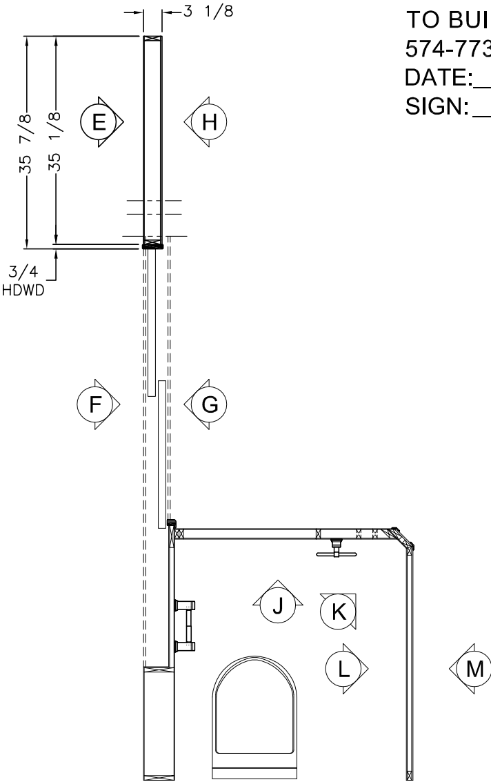
PLAN VIEW
