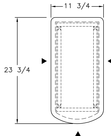
SOLID SURFACE ▶ — DENOTES A FINISHED EDGE
