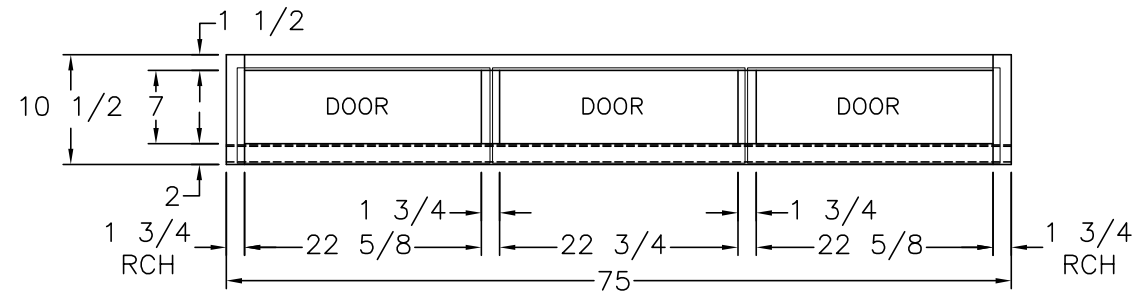
FRONT VIEW (3) 24 1/8x9 1/8 DOORS (TOP HG)
