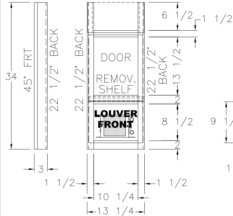
(1) 12 1/2x15 1/4 DOOR (LT HG) (1) 12 1/2x8 1/2 LOUVERED FRONT
