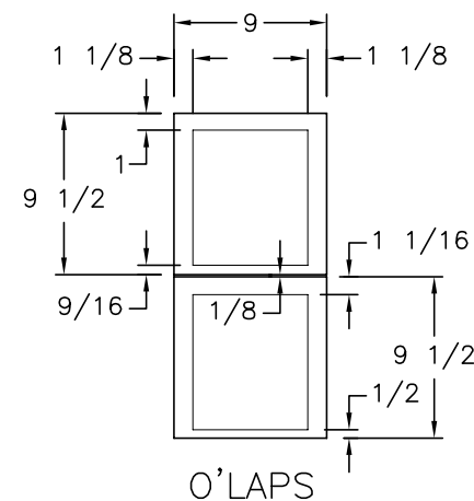
O'LAPS (2) 9 1/2x9 FRONTS
