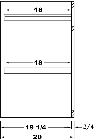
SIDE SECTION (B)
