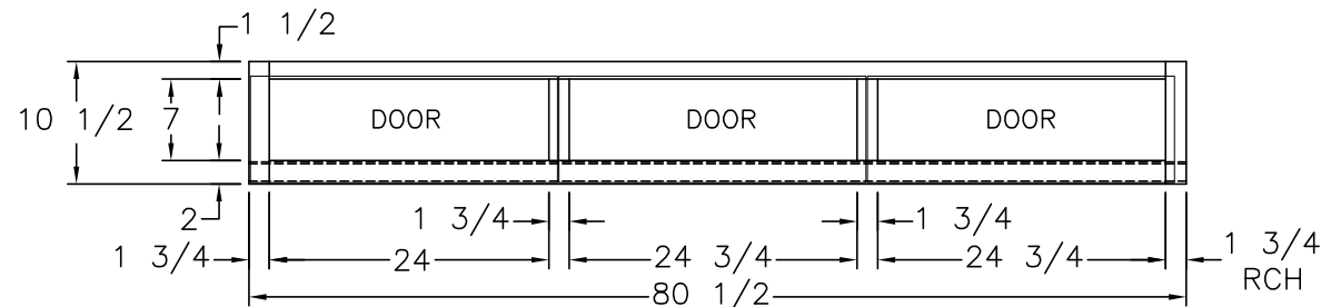
FRONT VIEW (3) 26 3/8x9 1/8 DOORS (TOP HG)
