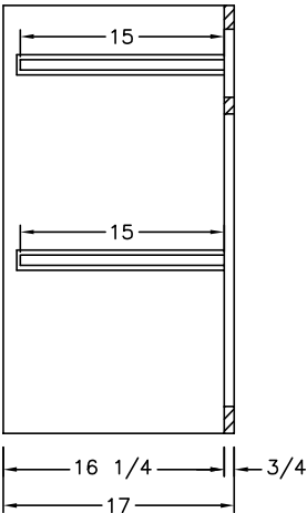
SIDE SECTION (B)
