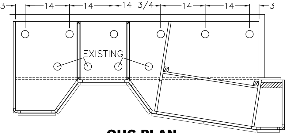
OHC PLAN
