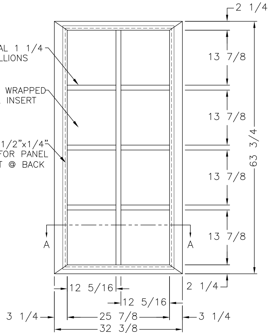
SLIDING DOOR (2) REQ'D
