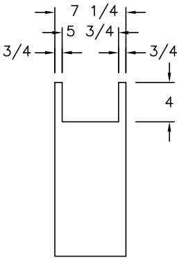
BACK PANEL
