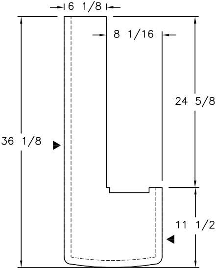
CHEST TOP 1/2" SOLID SURFACE ▲ — DENOTES A FINISHED EDGE
