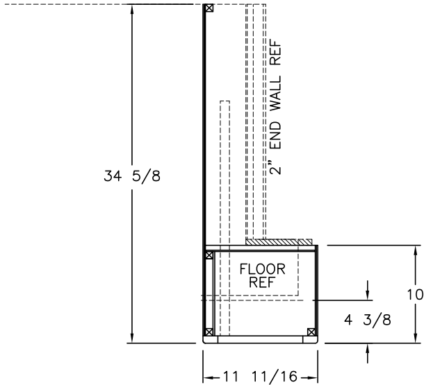
REAR CHEST TOP VIEW
