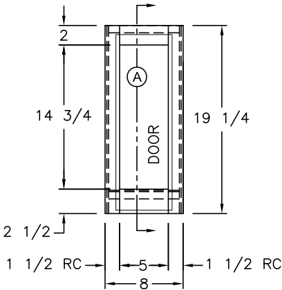
(1) 6x18 DOOR OVERHANG AT BOTTOM
