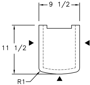
TOP VIEW 1/2 SOLID SURFACE
