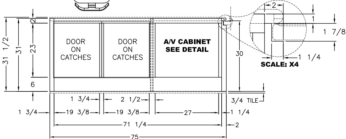
FRONT VIEW (FRAME)
