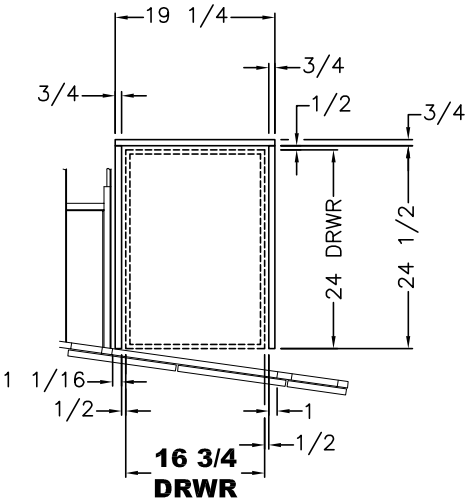
VIEW B DRAWER DETAIL
