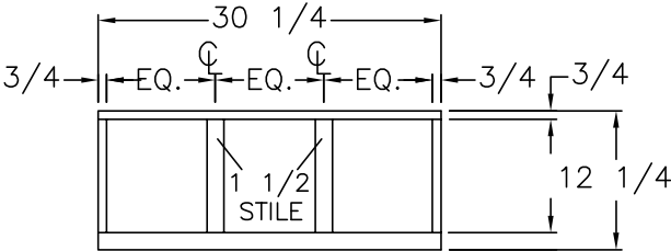
FRONT MICROWAVE SHELF DO NOT PANEL BOTTOM
