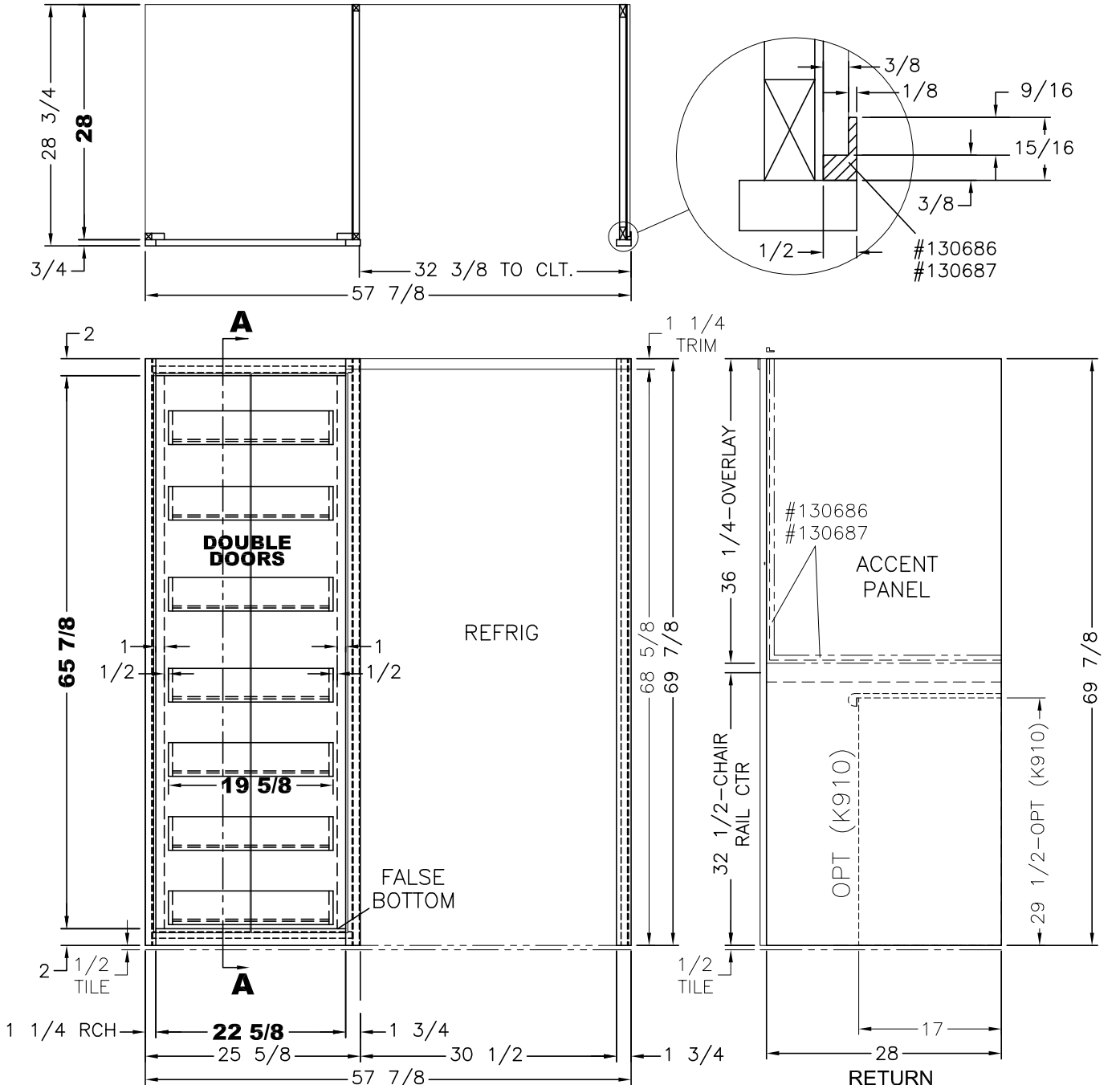
FRONT VIEW
