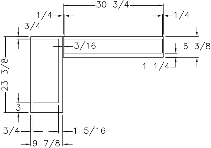
VIEW B OVERLAPS
