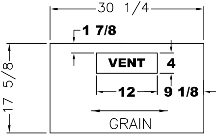
5/8 PLYWOOD DETAIL
