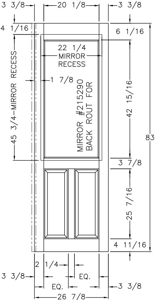
VIEW (B)
