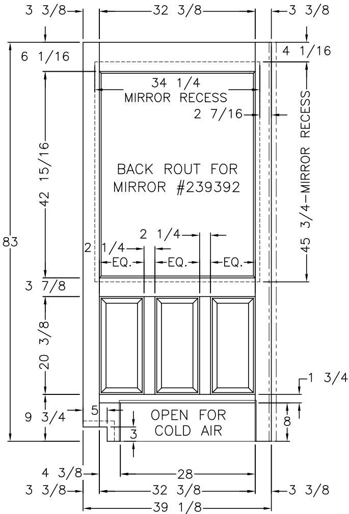
VIEW 'B' PANEL OVERLAY
