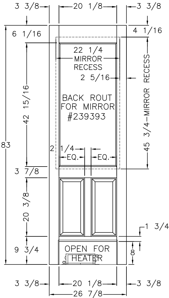
VIEW 'D' PANEL OVERLAY
