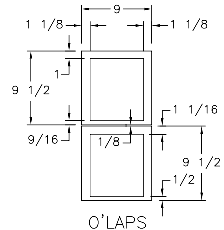
(2) 9 1/2x9 FRONTS
