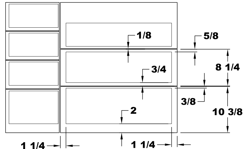
VIEW A OVERLAPS
