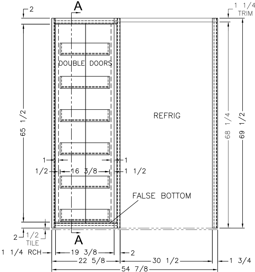
FRONT VIEW
