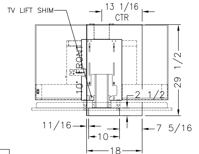
FRONT VIEW 3/4" MOUNTING PANEL
