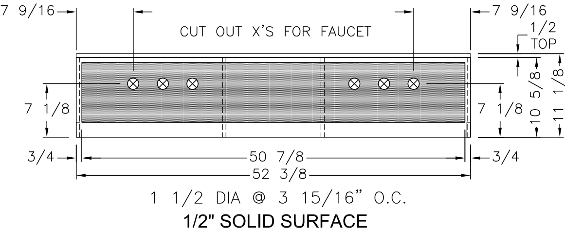
SPLASH (FRONT VIEW) SHADED DENOTES 1/4" RECESS FOR TILE INLAY
