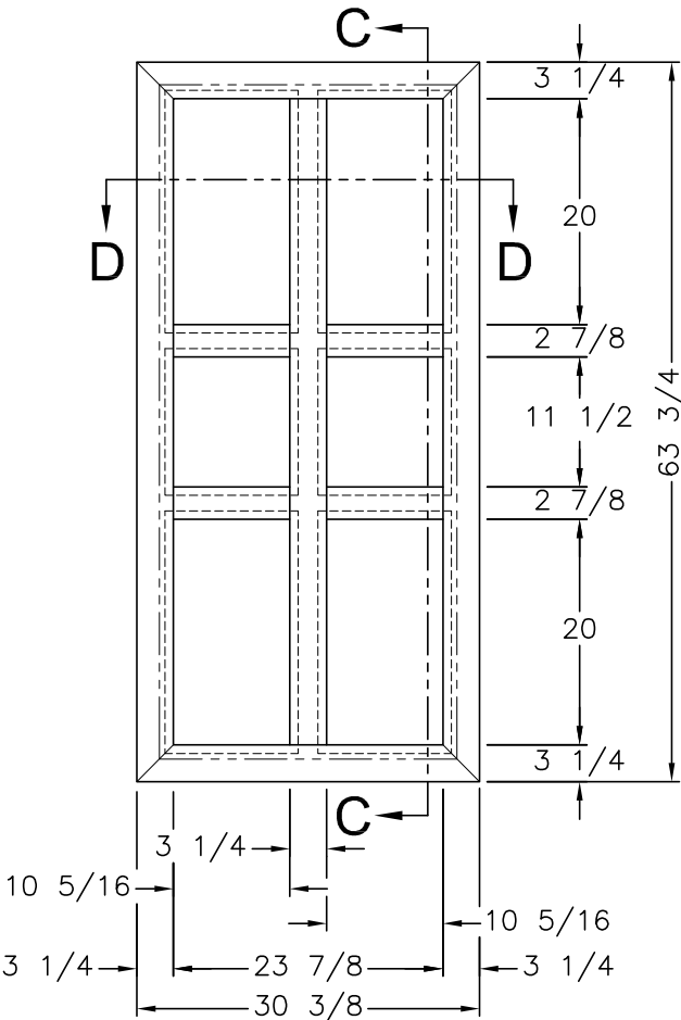
SLIDING DOOR (2) REQ'D
