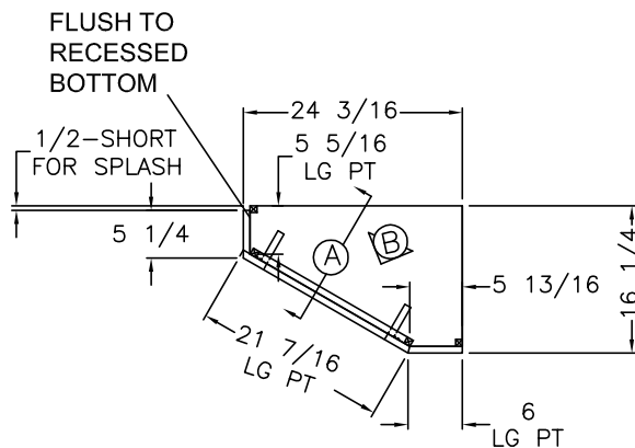
TOP VIEW 16 7/16Wx14 3/4H TAMBOUR DOOR
