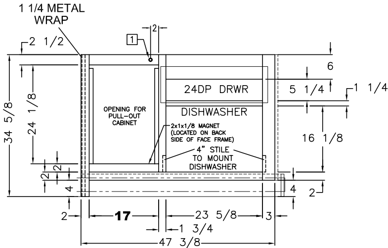
VIEW A (1) 8 7/8x26 1/8 DRAWER FRONT
