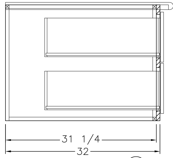
SIDE SECTION (A)
