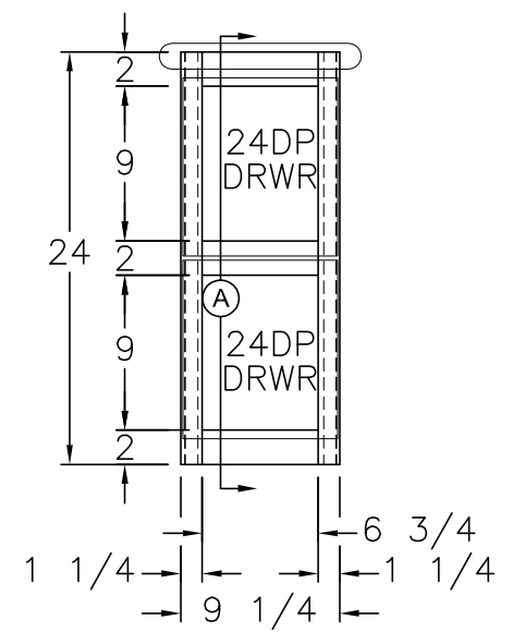
FRONT VIEW (2) 10 3/8x9 FRONTS
