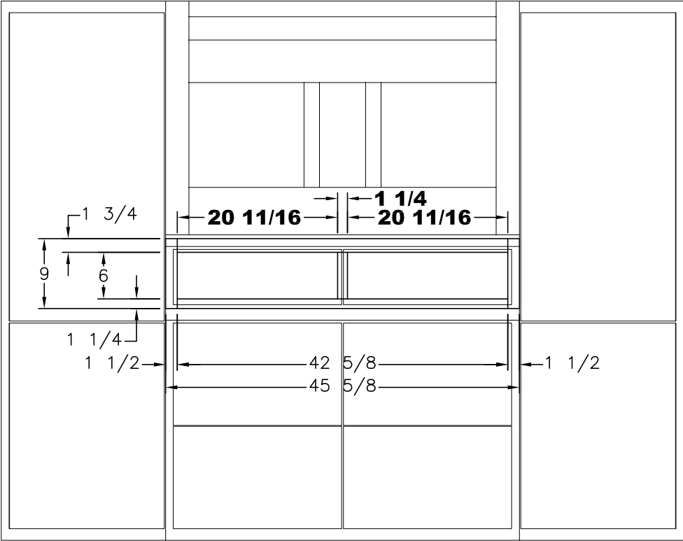
FRONT
