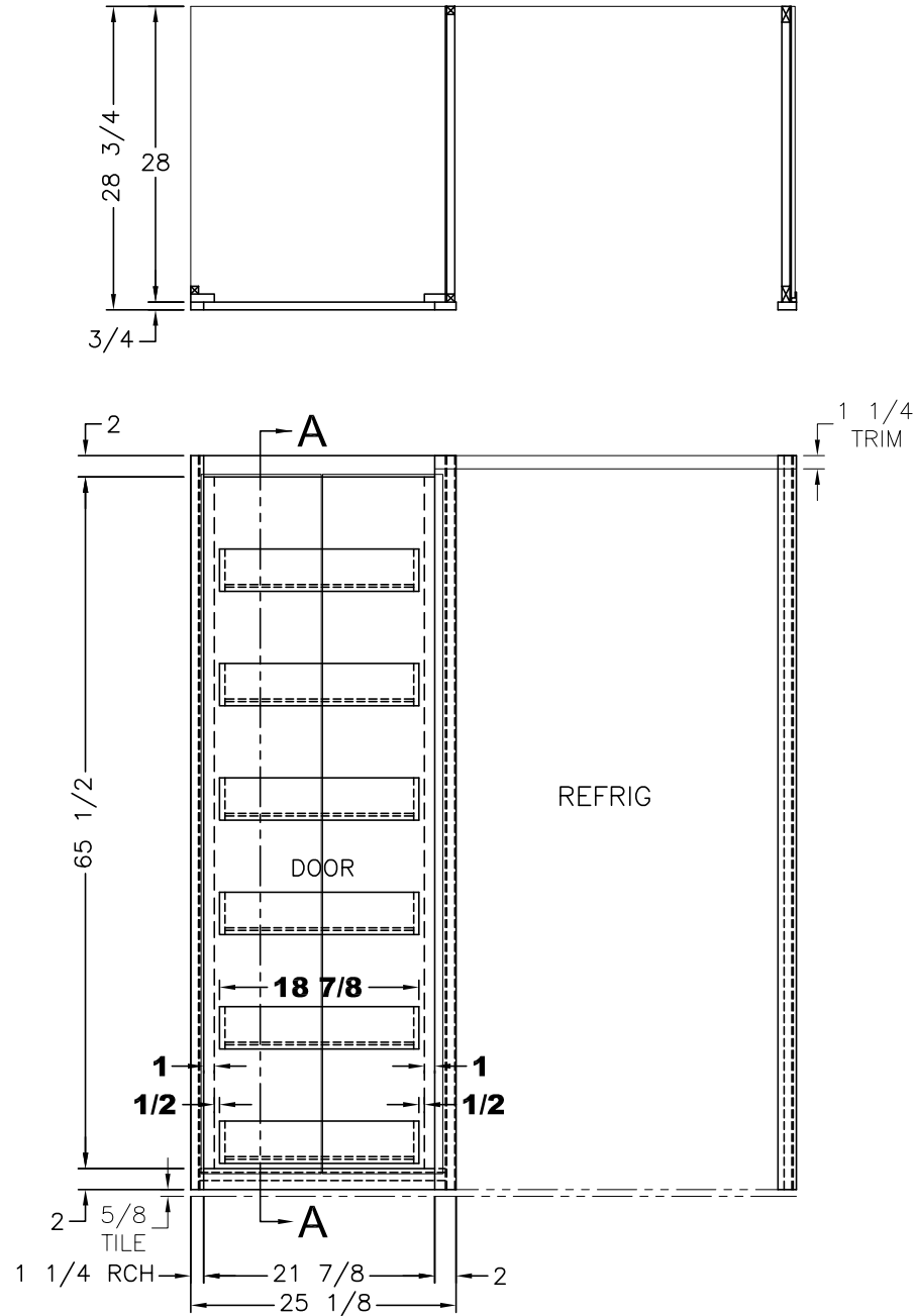
FRONT VIEW
