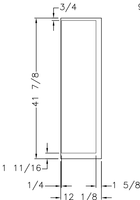
PANTRY OVERLAPS
