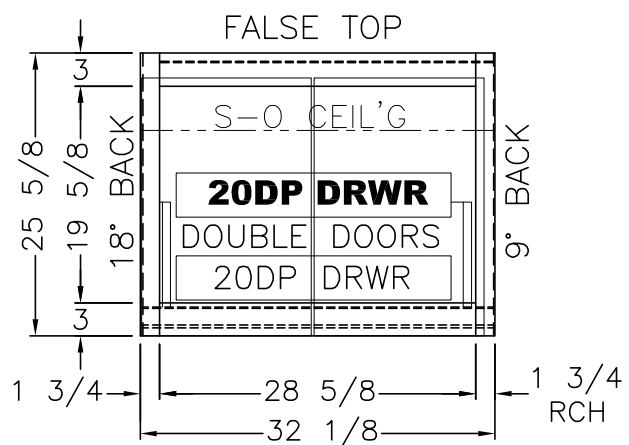
(2) 15 3/8x23 3/8 DOORS
