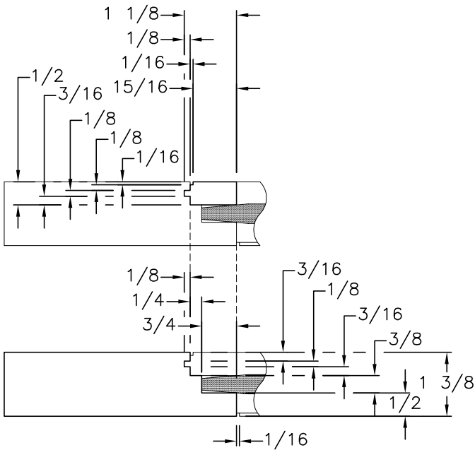
TYPICAL CUTS
