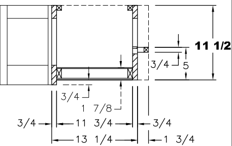
SECTION A
