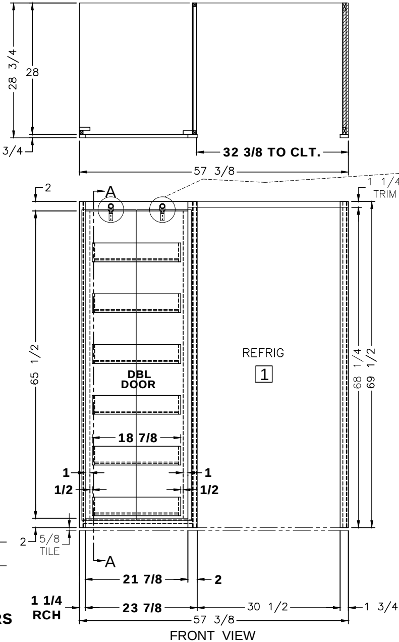
FRONT VIEW
