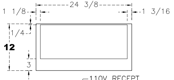
(1) 24 3/8x12 DOOR
