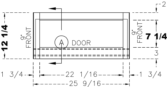
(1) 24 3/8x12 DOOR
