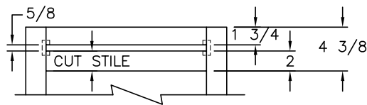
CABINET BASE FRONT VIEW
