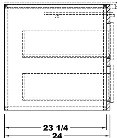
SIDE SECTION (A)
