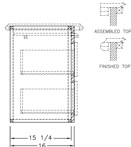
SIDE SECTION (A)
