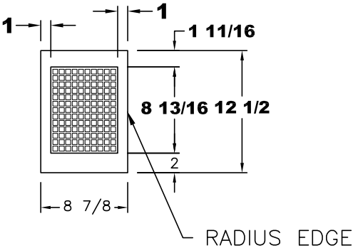
VIEW (C)
