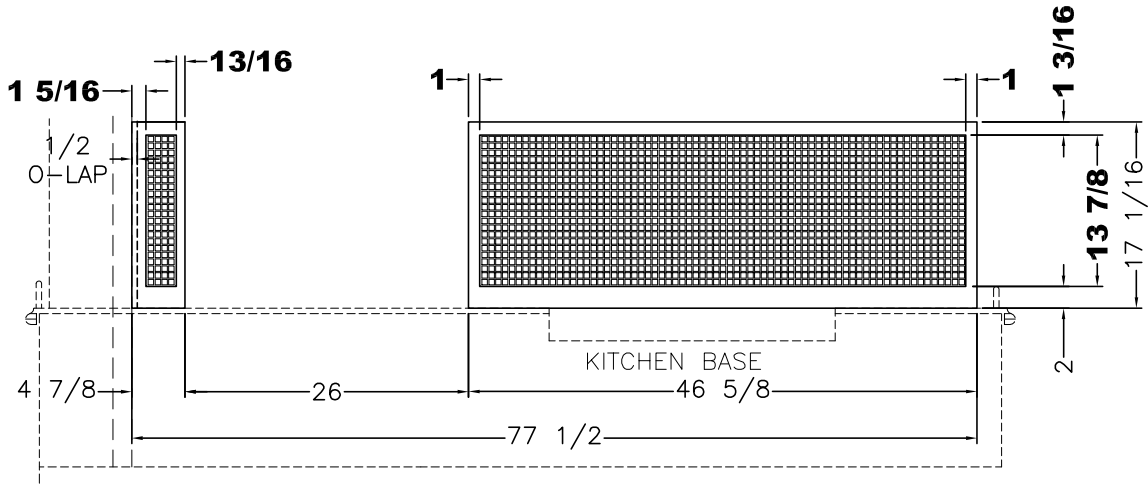
MAIN PANEL PIECE
