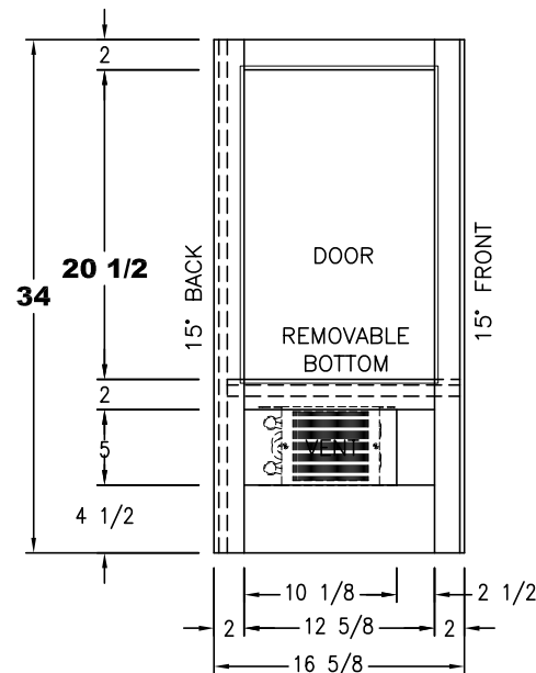
VIEW (B)
