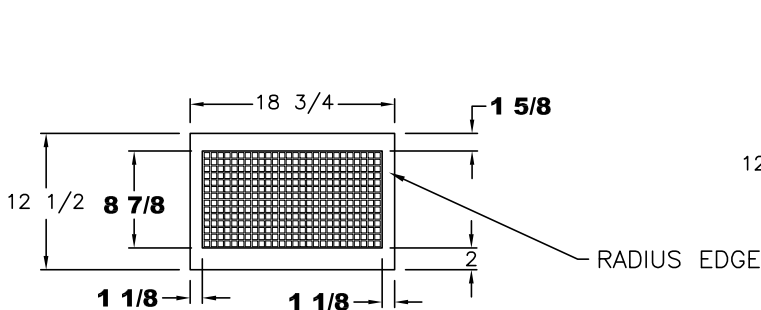
BACK SPLASH (A)
