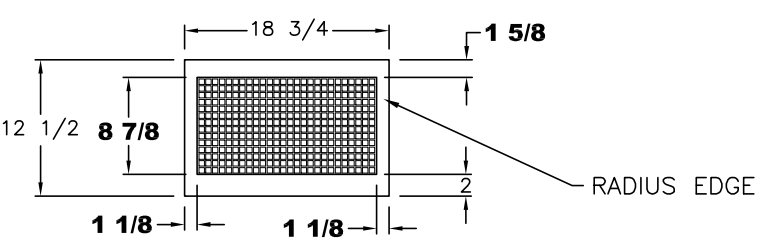
BACK SPLASH (C)
