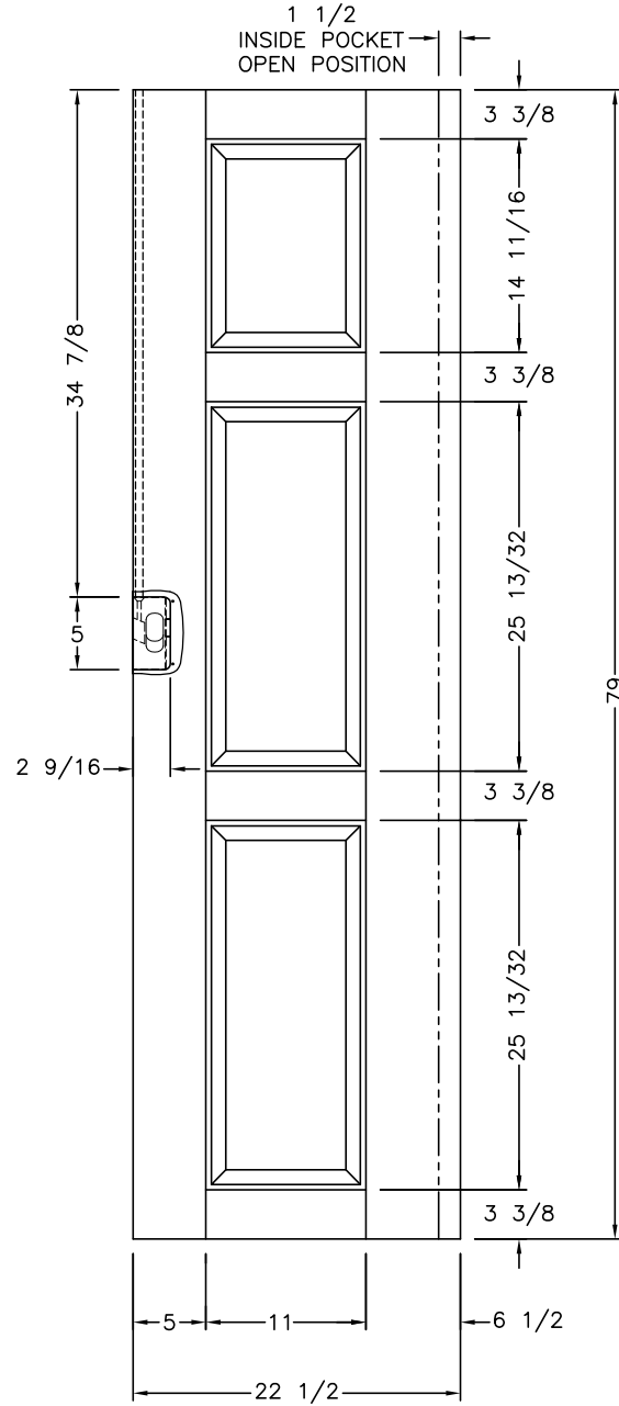
KITCHEN SIDE
