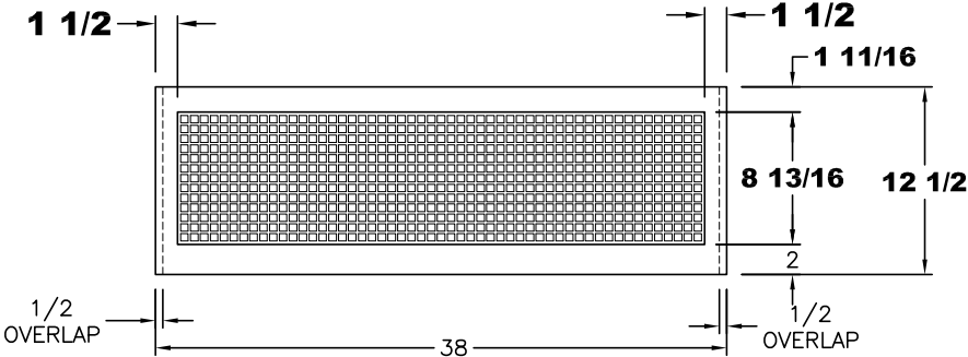
VIEW (B)
