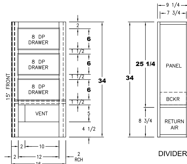
VIEW (C)
