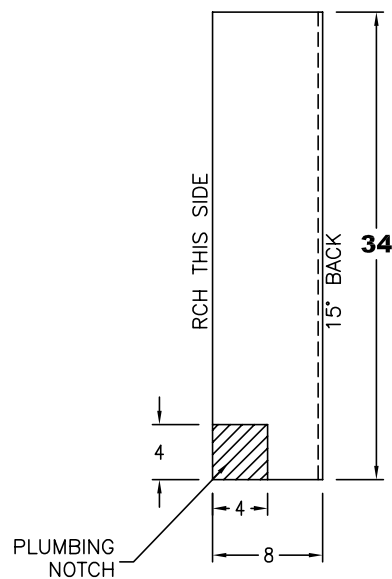
VIEW (A)
