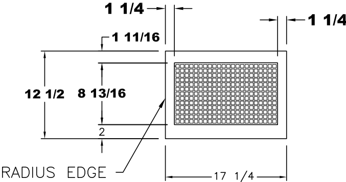
VIEW (A)
