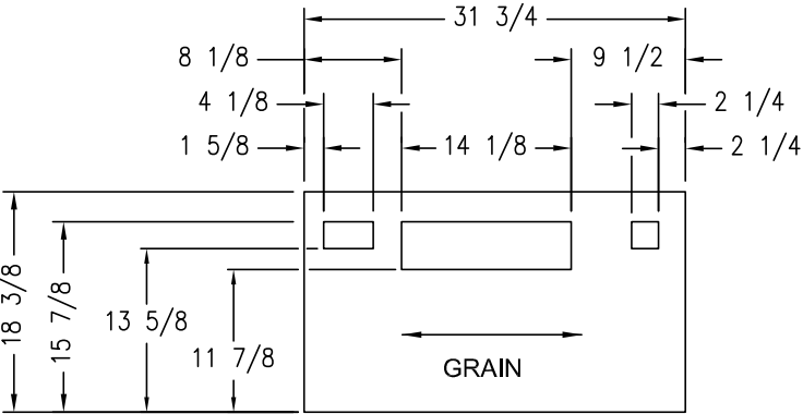
5/8 PLYWOOD DETAIL DETAIL 'F'
