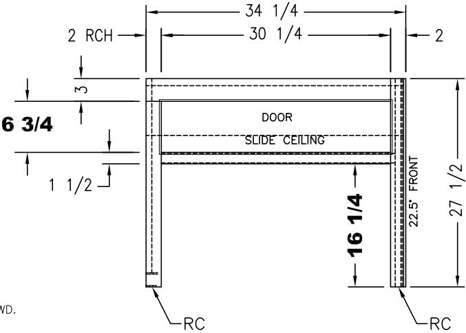
(1) 7 1/4 X 30 3/4 FALSE FRONT VIEW (A)
