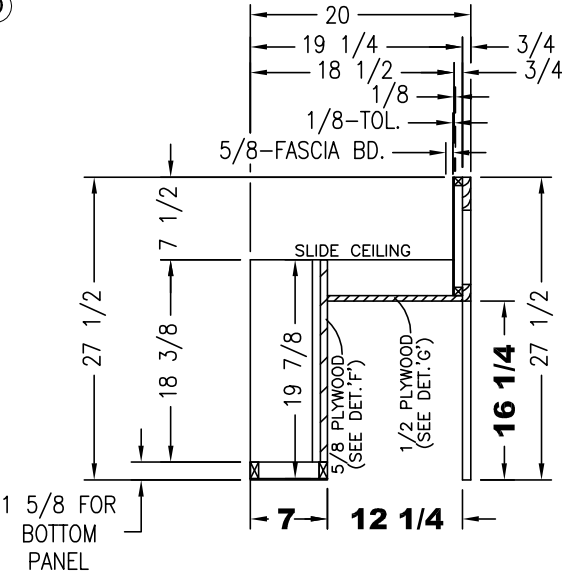
SIDE SECTION (A)
