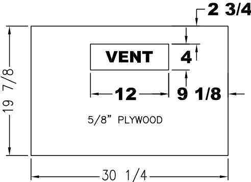
DETAIL 'F'
