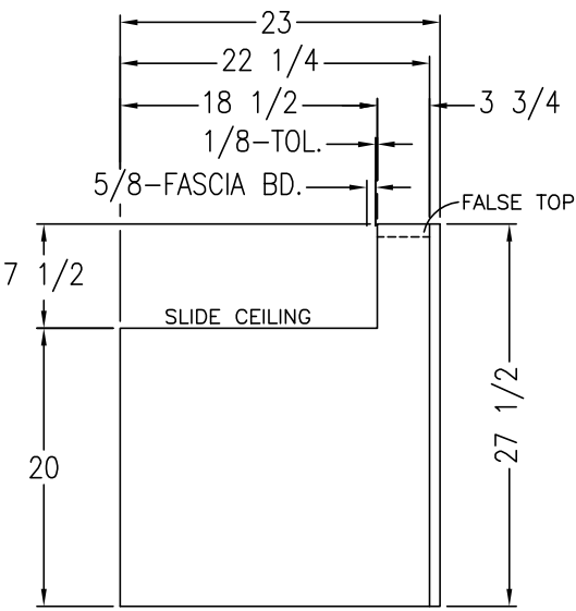
VIEW (A)
