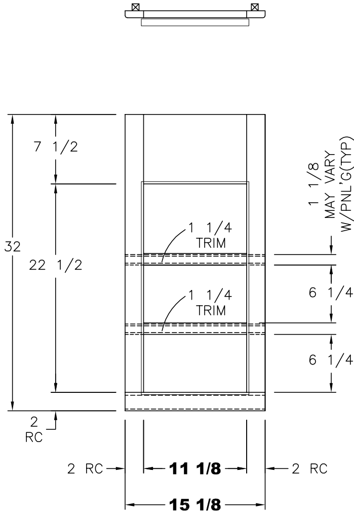
VIEW A
