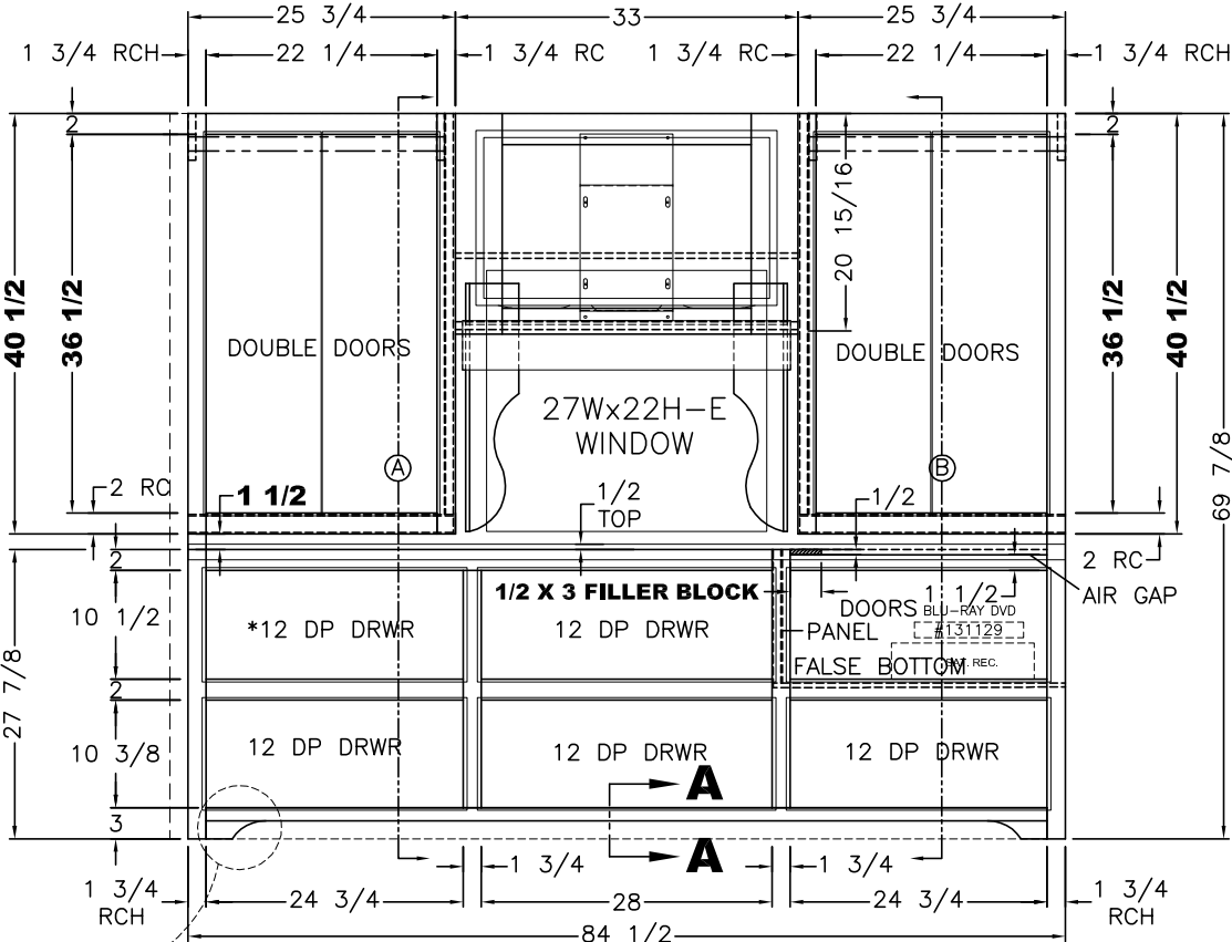
FRONT VIEW
