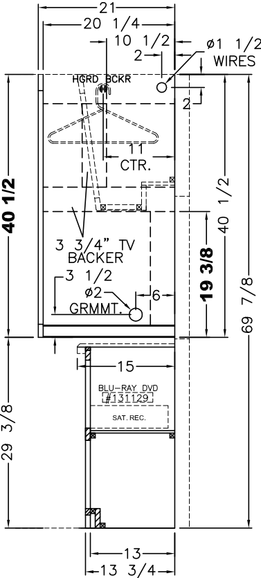
SECTION (B)
