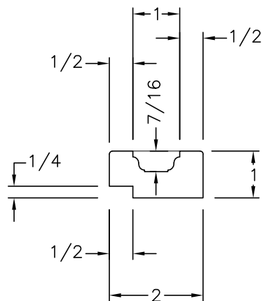
SECTION B-B 4X SCALE
