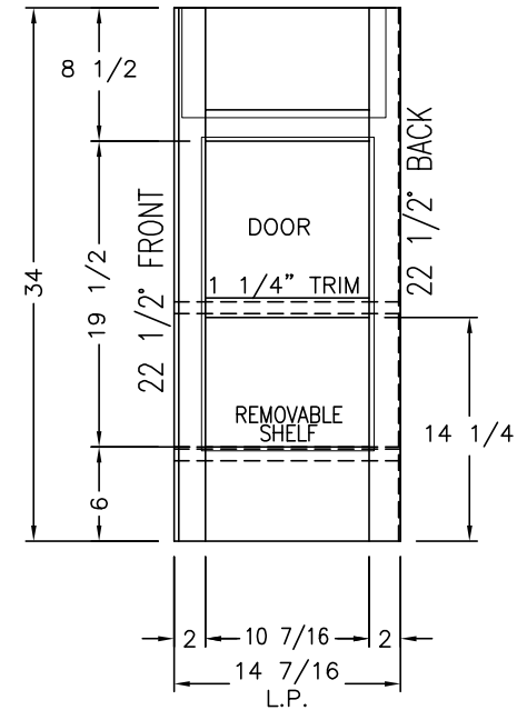
VIEW (B)
