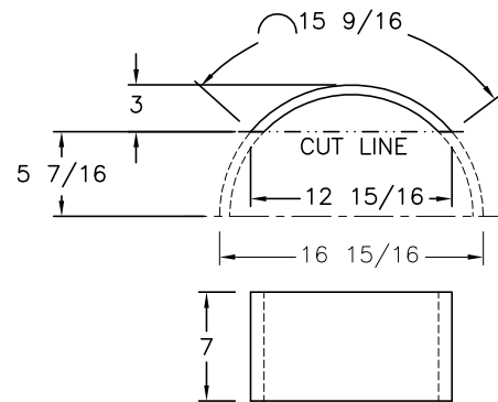
APRON DETAIL
