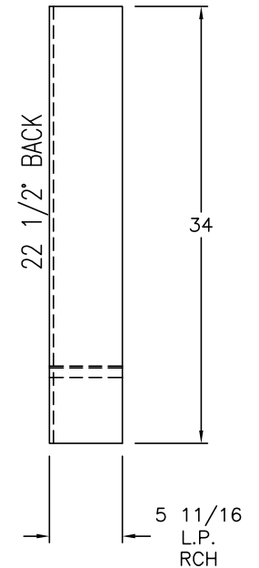
VIEW ©
