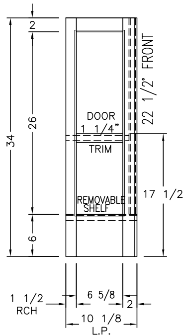
VIEW (A)
