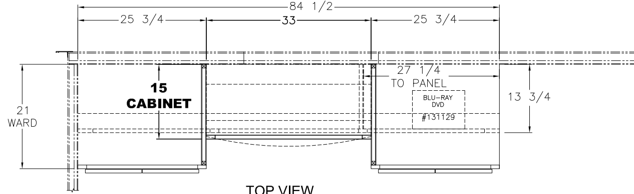
TOP VIEW
