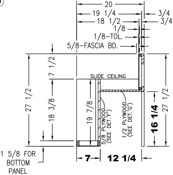
SIDE SECTION (A)
