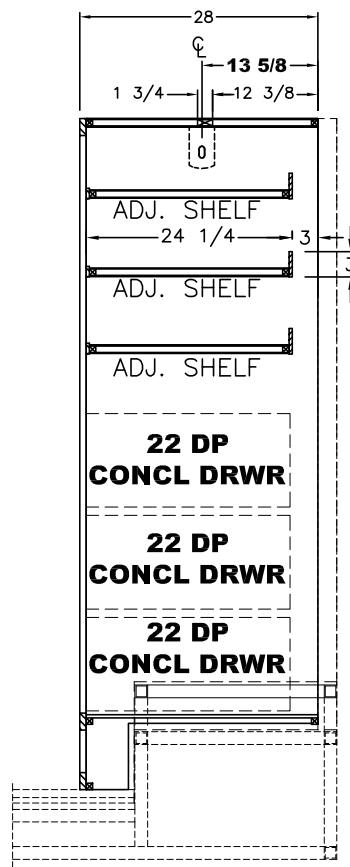
SECTION VIEW (A)
