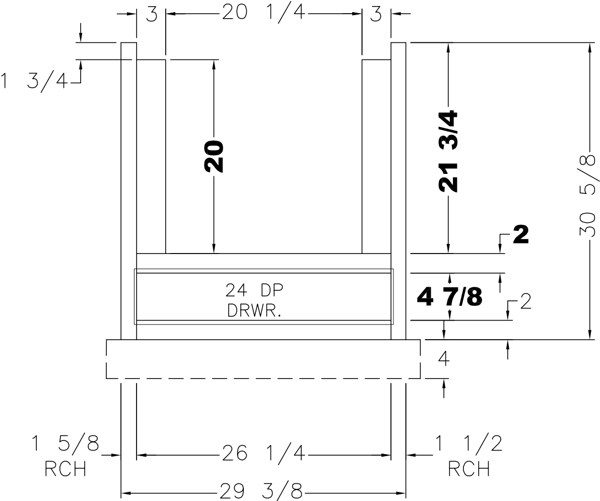
VIEW (C) (1) 5 3/4x26 3/4 FRONT
