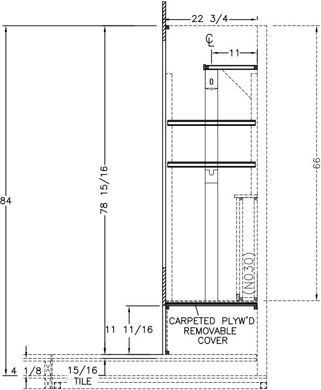
SECTION VIEW C
