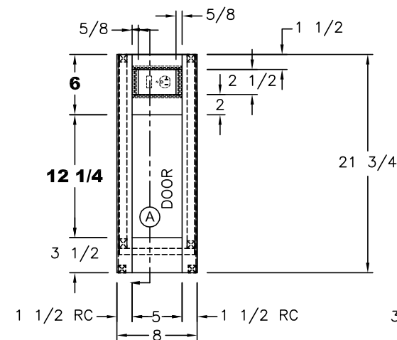
(1) 5 3/4x15 3/4 DOOR OVERHANG AT BOTTOM
