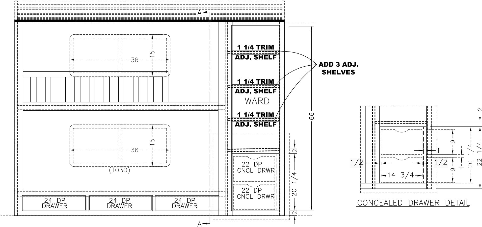
FRONT VIEW
