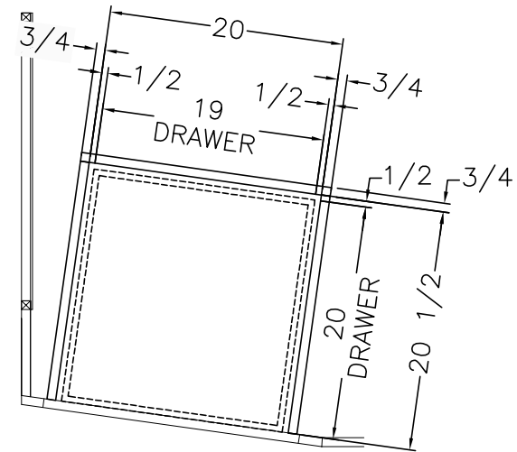
VIEW E DRAWER DETAIL
